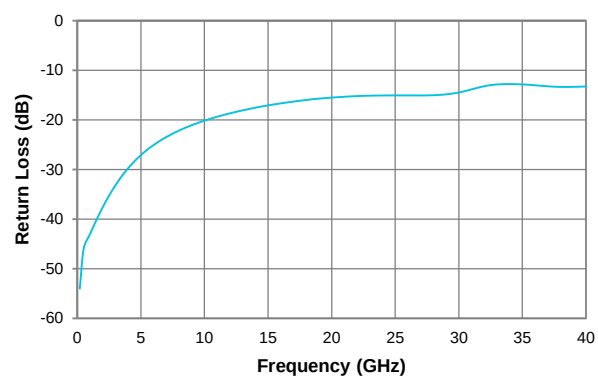
Return Loss
